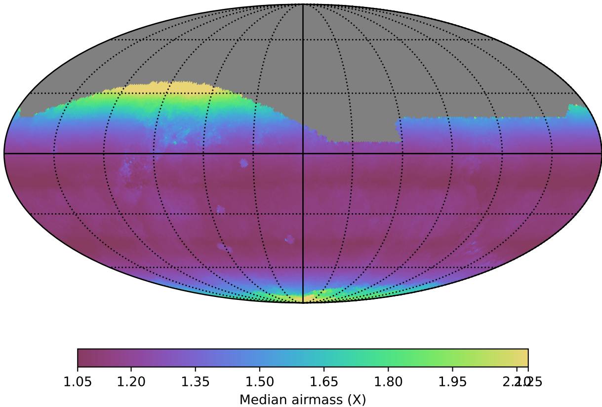
too_5_1v3.4_10yrs All sky r band: Median airmass
