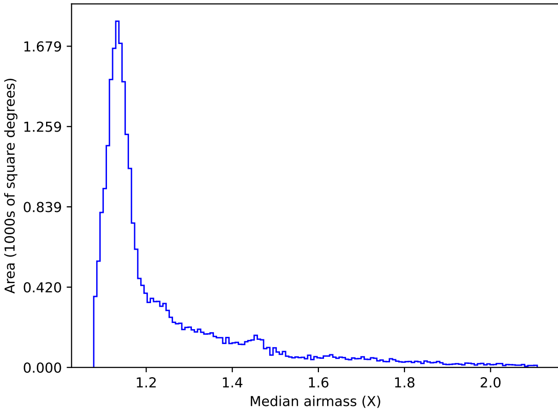
too_5_1v3.4_10yrs All sky i band: Median airmass
