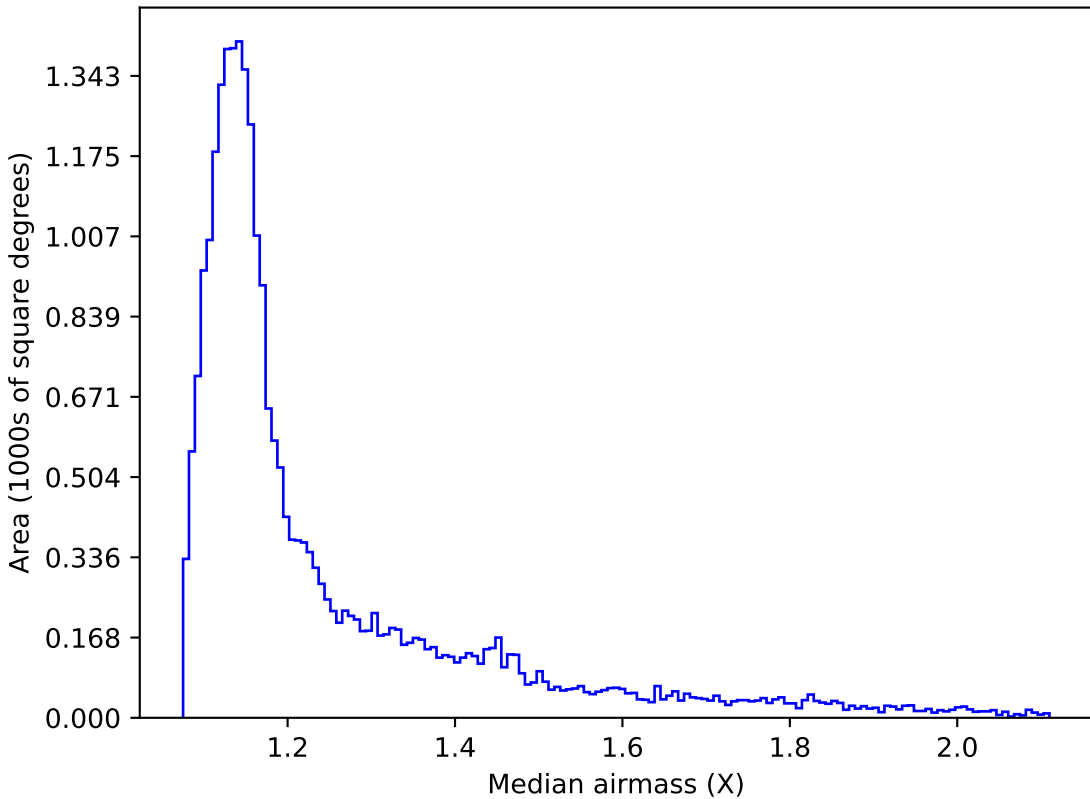
too_5_1v3.4_10yrs All sky g band: Median airmass
