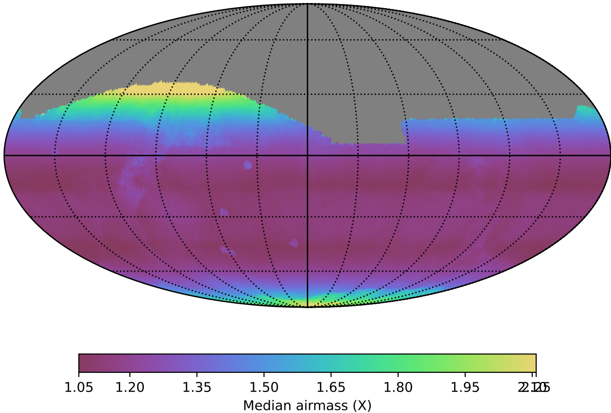
too_5_1v3.4_10yrs All sky all bands: Median airmass
