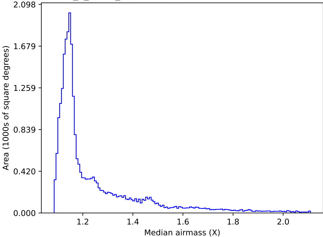
too_5_1v3.4_10yrs All sky all bands: Median airmass
