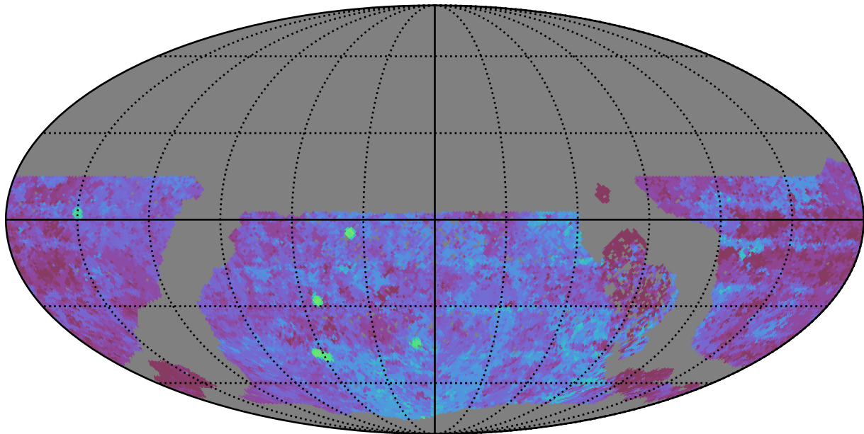
too_5_1v3.4_10yrs WFD u band: Median Season Length
