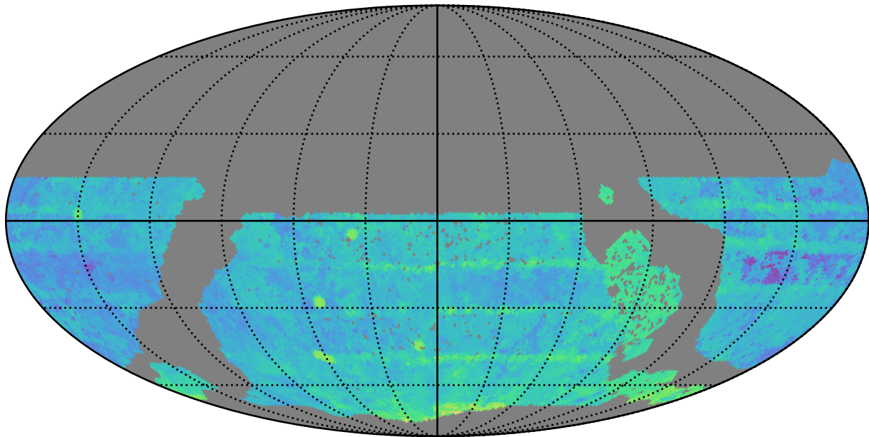
too_5_1v3.4_10yrs WFD r band: Median Season Length
