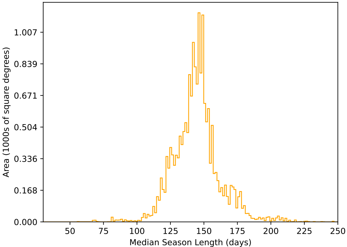
too_5_1v3.4_10yrs WFD r band: Median Season Length
