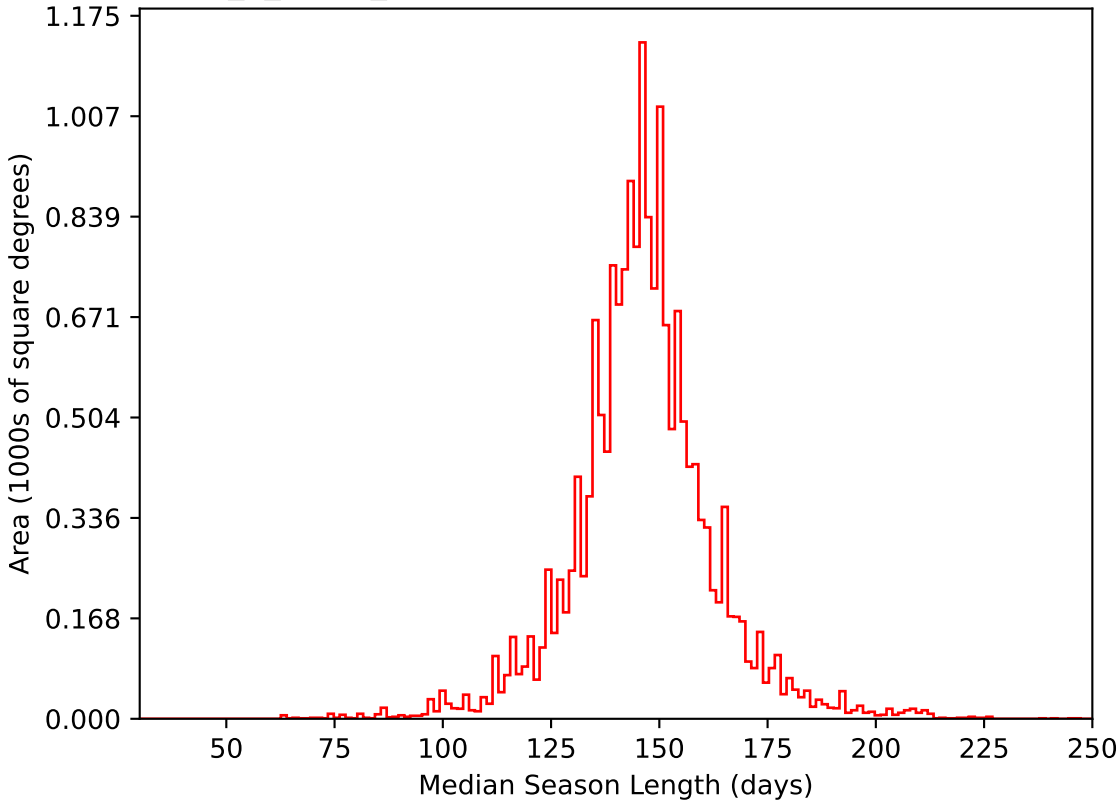
too_5_1v3.4_10yrs WFD i band: Median Season Length
