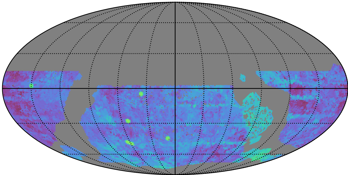
too_5_1v3.4_10yrs WFD g band: Median Season Length
