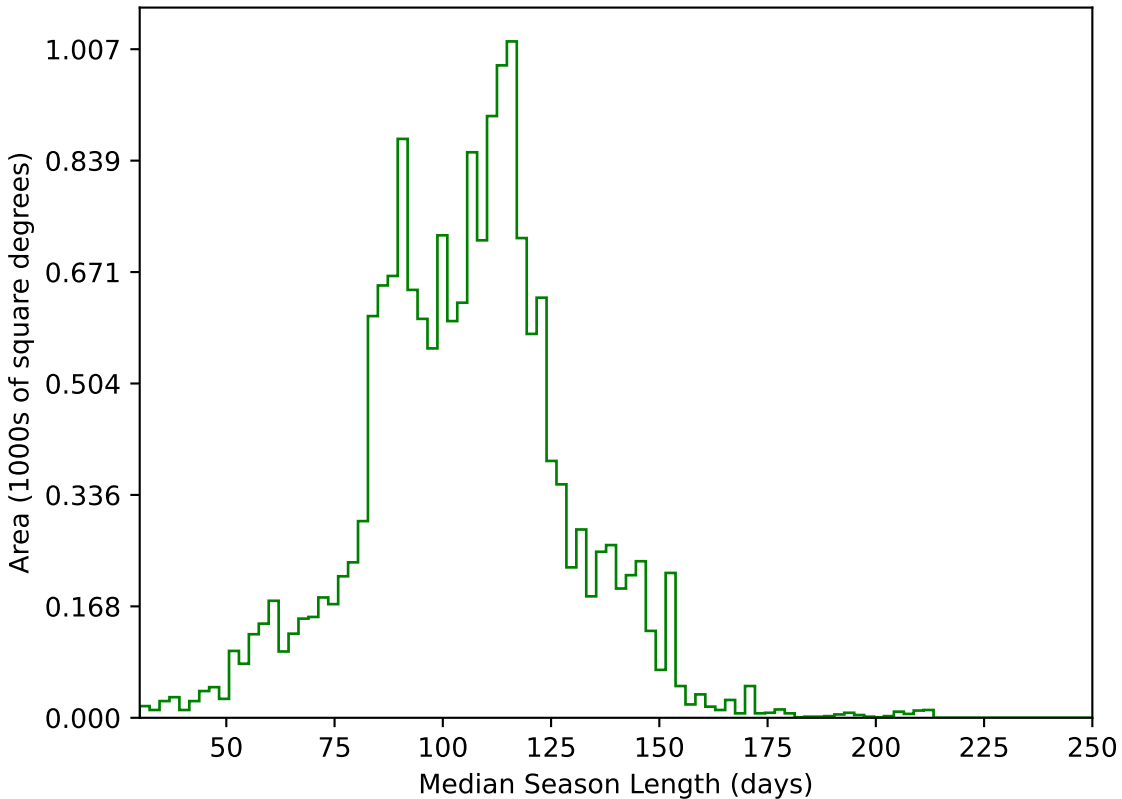
too_5_1v3.4_10yrs WFD g band: Median Season Length
