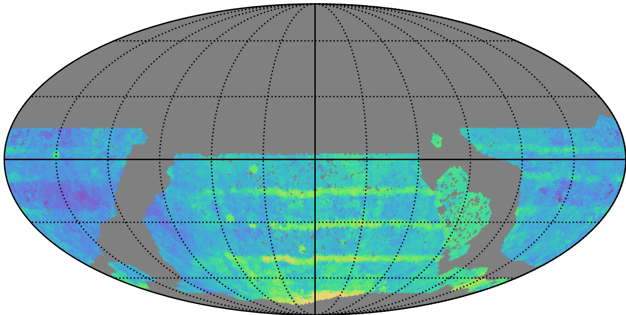
too_5_1v3.4_10yrs WFD all bands: Median Season Length
