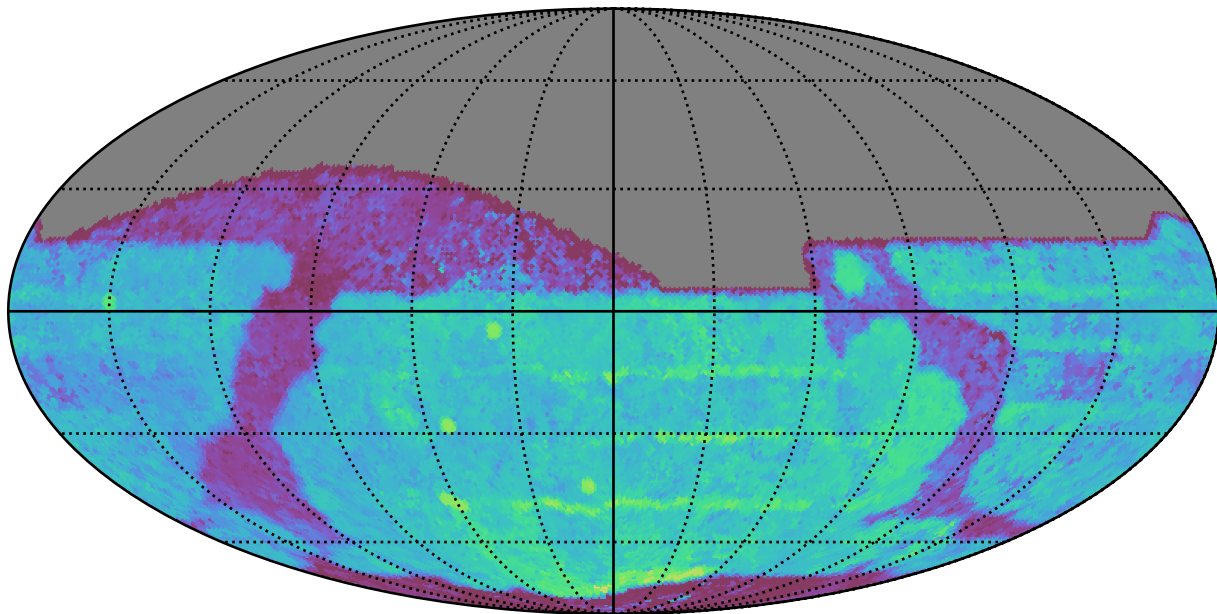
too_5_1v3.4_10yrs All sky z band: Median Season Length
