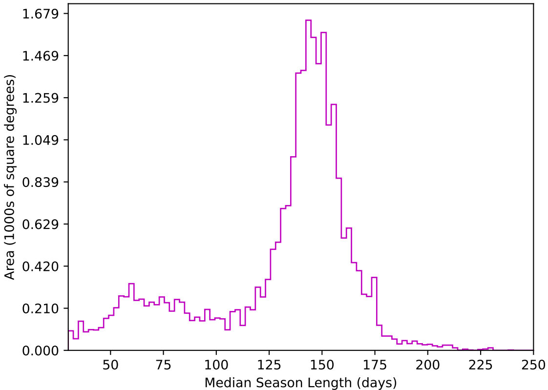
too_5_1v3.4_10yrs All sky z band: Median Season Length
