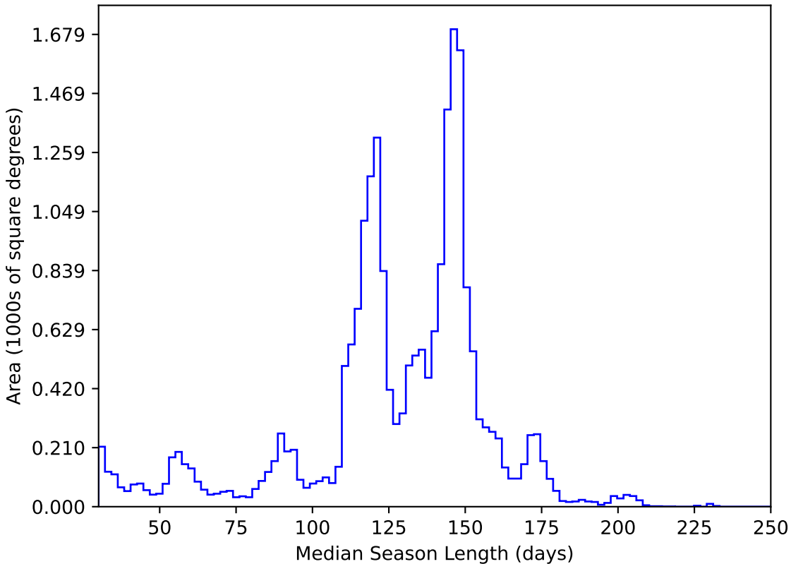
too_5_1v3.4_10yrs All sky y band: Median Season Length
