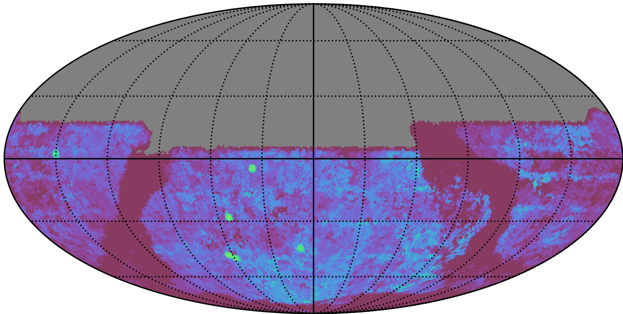
too_5_1v3.4_10yrs All sky u band: Median Season Length
