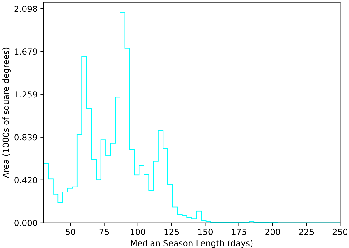
too_5_1v3.4_10yrs All sky u band: Median Season Length
