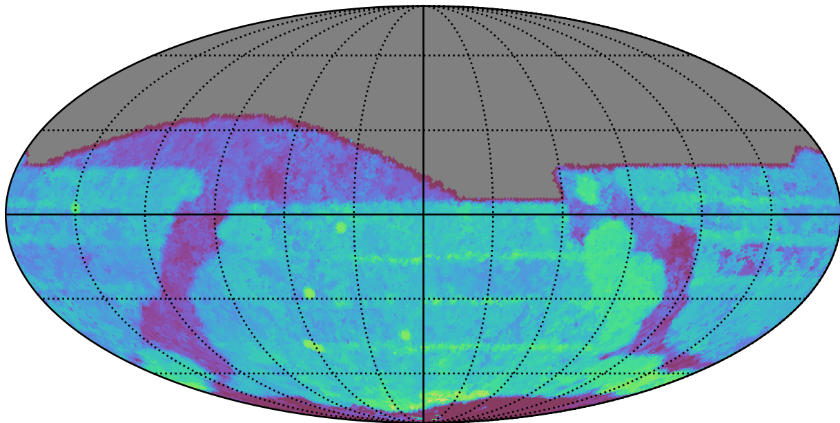
too_5_1v3.4_10yrs All sky r band: Median Season Length
