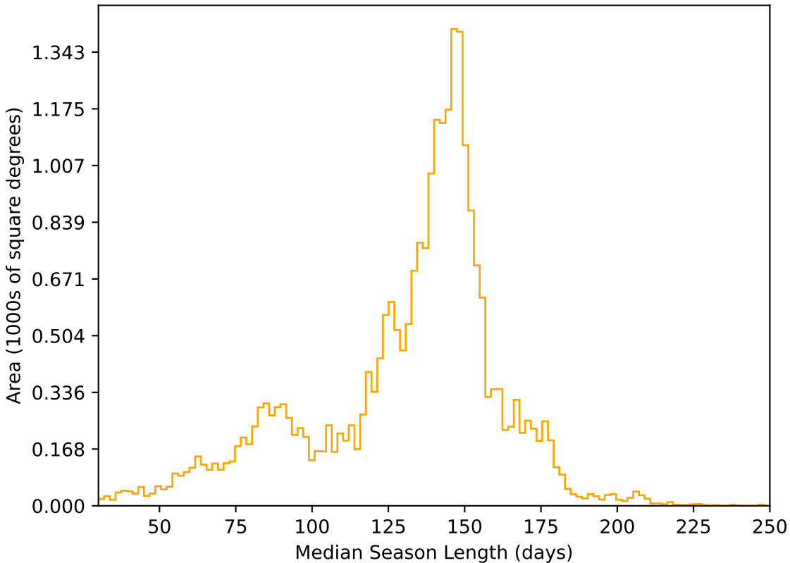
too_5_1v3.4_10yrs All sky r band: Median Season Length
