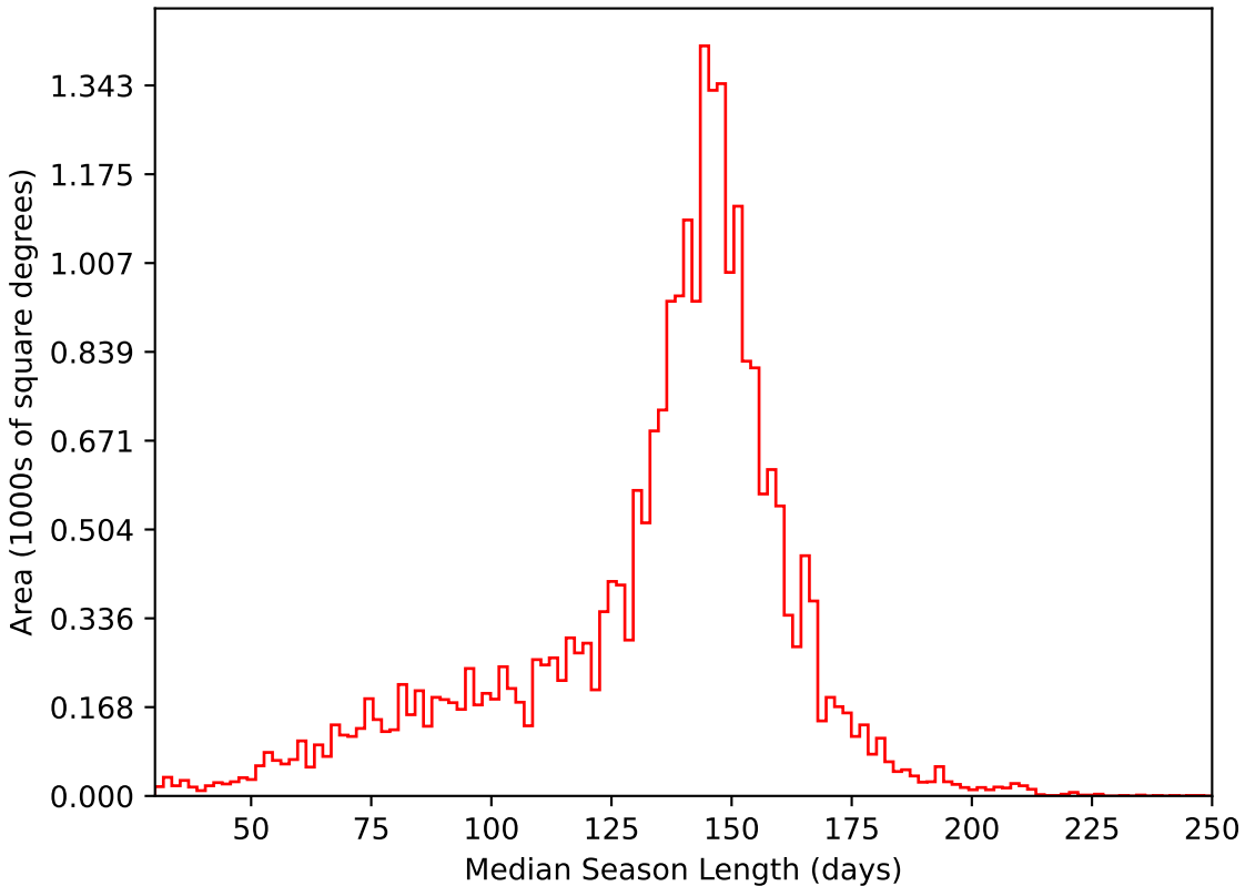
too_5_1v3.4_10yrs All sky i band: Median Season Length
