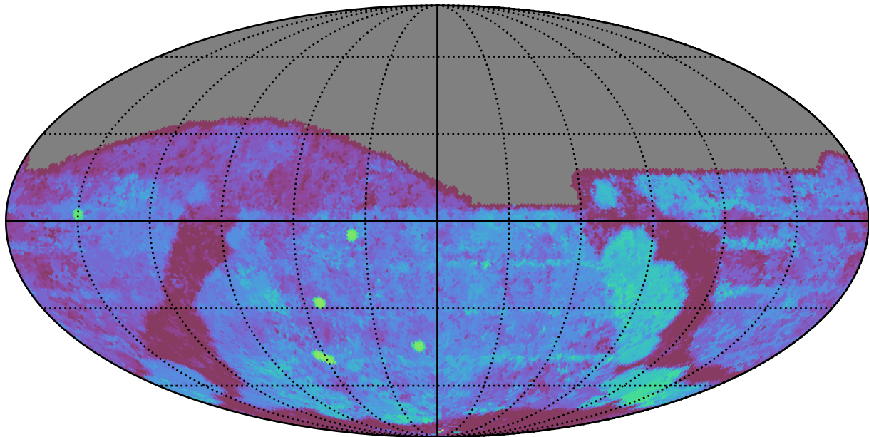
too_5_1v3.4_10yrs All sky g band: Median Season Length
