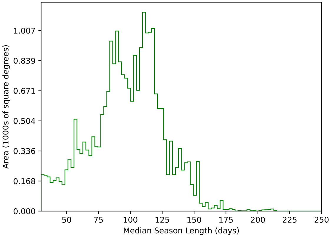
too_5_1v3.4_10yrs All sky g band: Median Season Length
