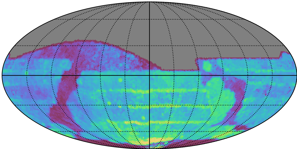
too_5_1v3.4_10yrs All sky all bands: Median Season Length
