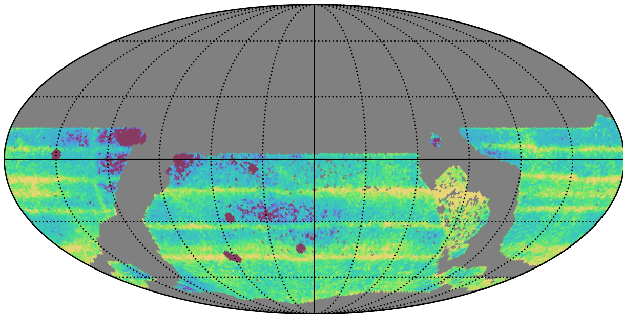
too_5_1v3.4_10yrs WFD: Median Intra-Night Gap
