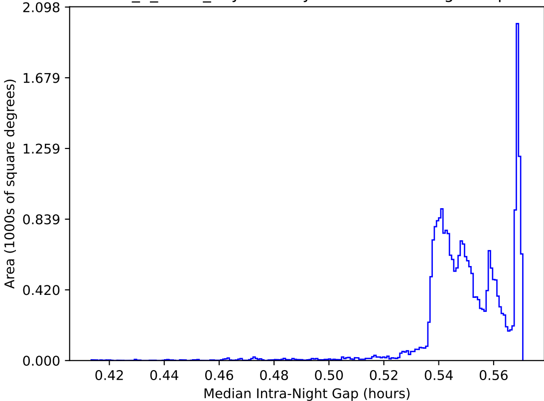
too_5_1v3.4_10yrs All sky: Median Intra-Night Gap
