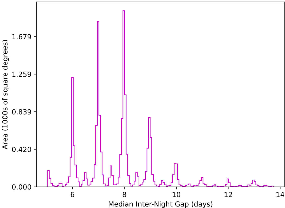
too_5_1v3.4_10yrs WFD z band: Median Inter-Night Gap
