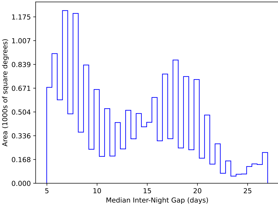
too_5_1v3.4_10yrs WFD y band: Median Inter-Night Gap
