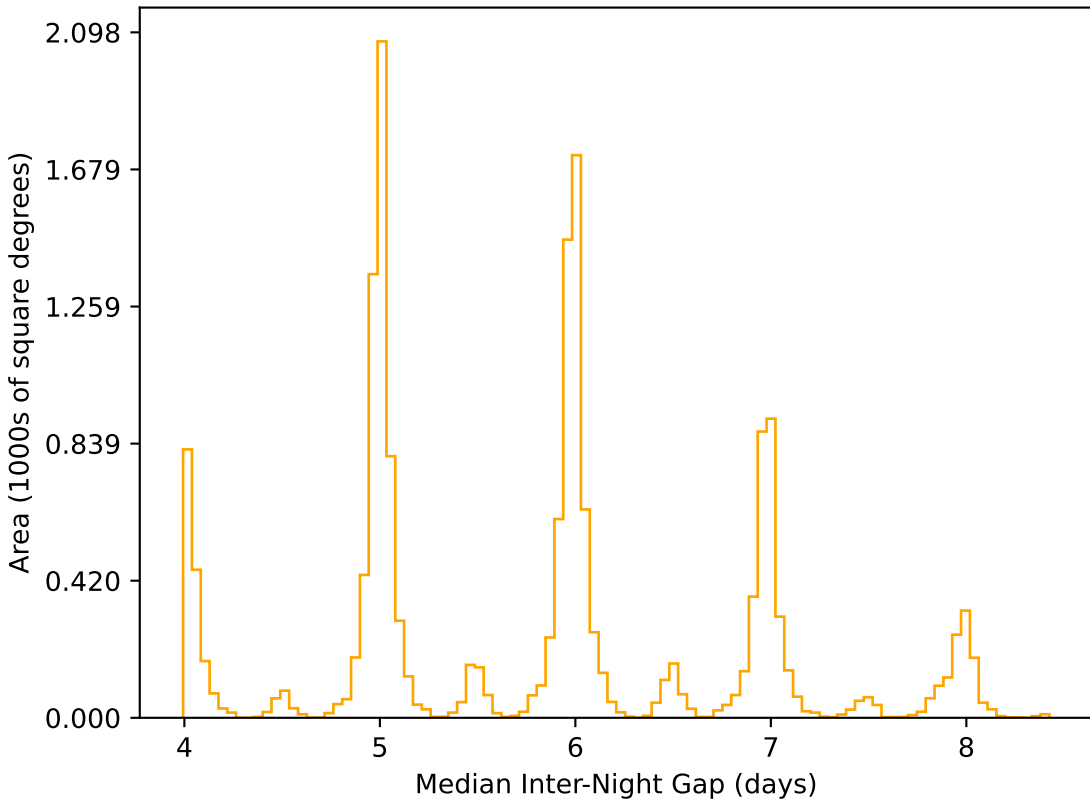
too_5_1v3.4_10yrs WFD r band: Median Inter-Night Gap
