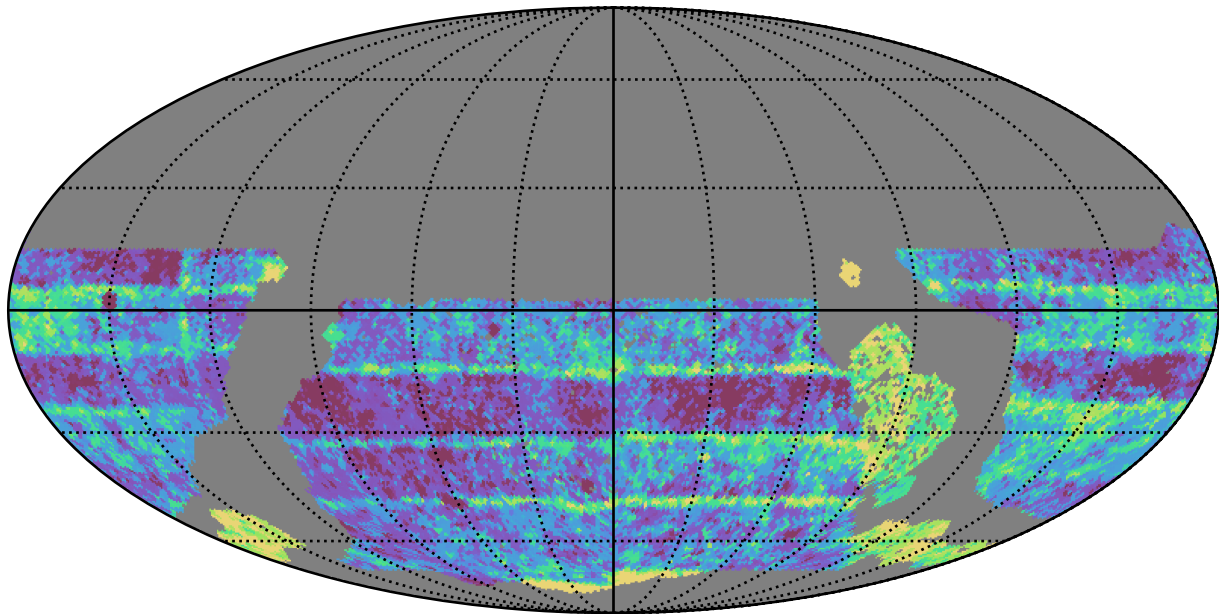
too_5_1v3.4_10yrs WFD i band: Median Inter-Night Gap
