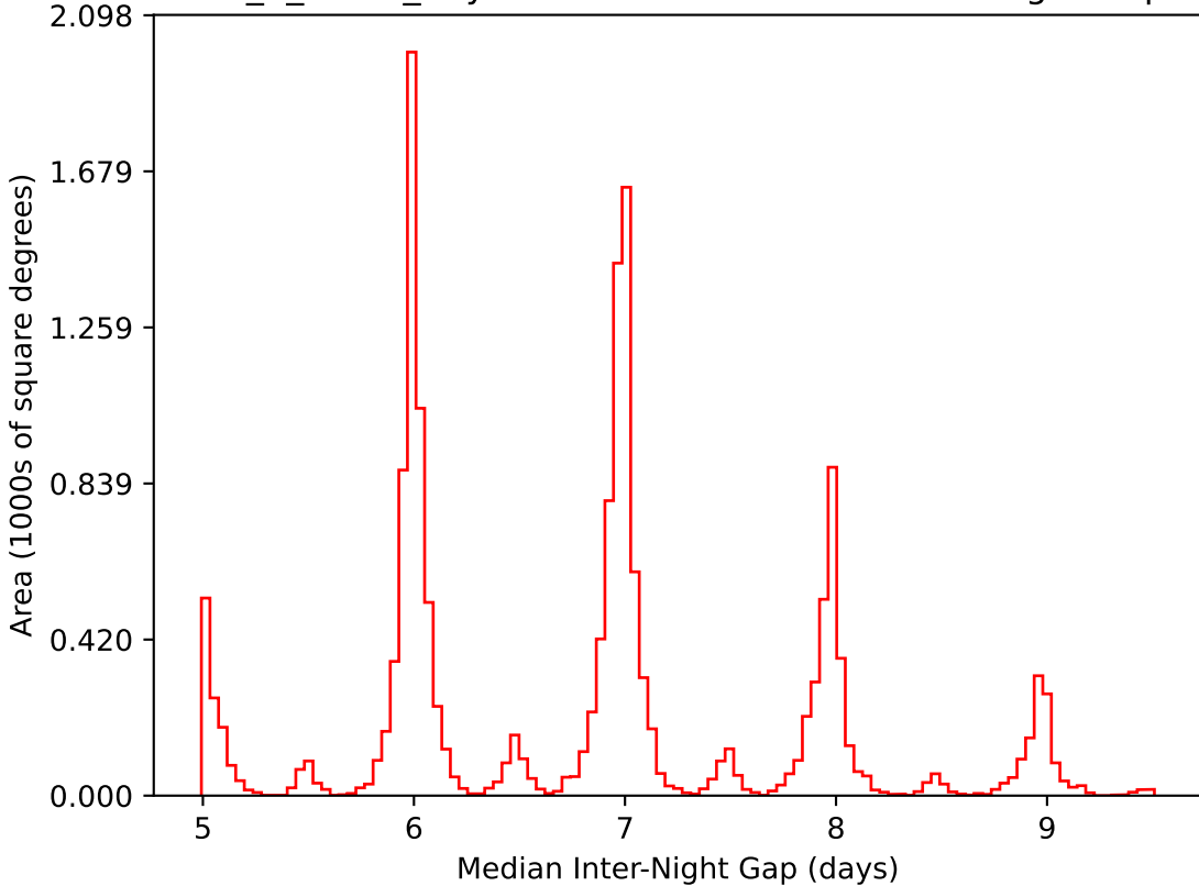
too_5_1v3.4_10yrs WFD i band: Median Inter-Night Gap
