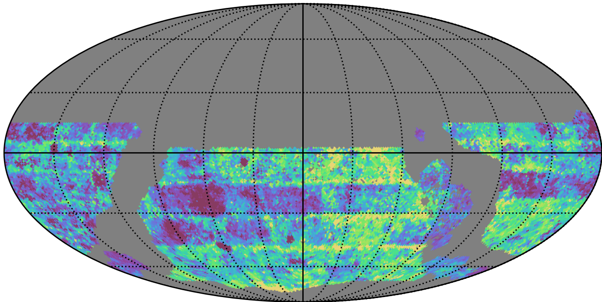
too_5_1v3.4_10yrs WFD g band: Median Inter-Night Gap
