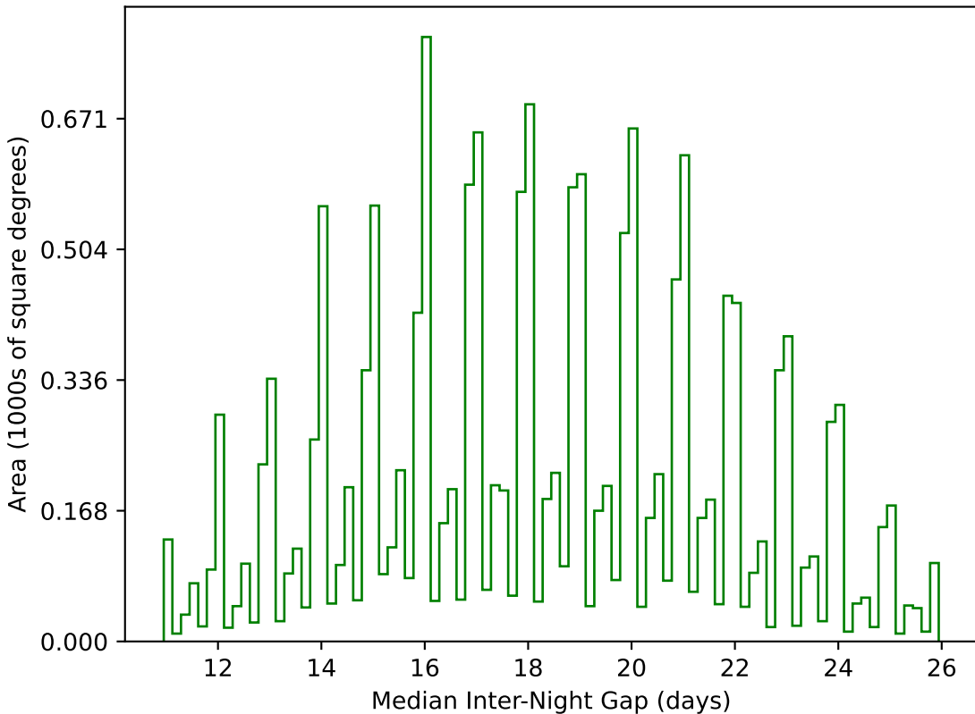
too_5_1v3.4_10yrs WFD g band: Median Inter-Night Gap
