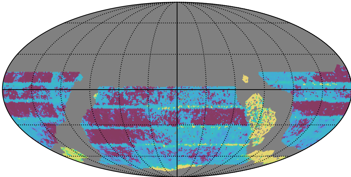
too_5_1v3.4_10yrs WFD all bands: Median Inter-Night Gap
