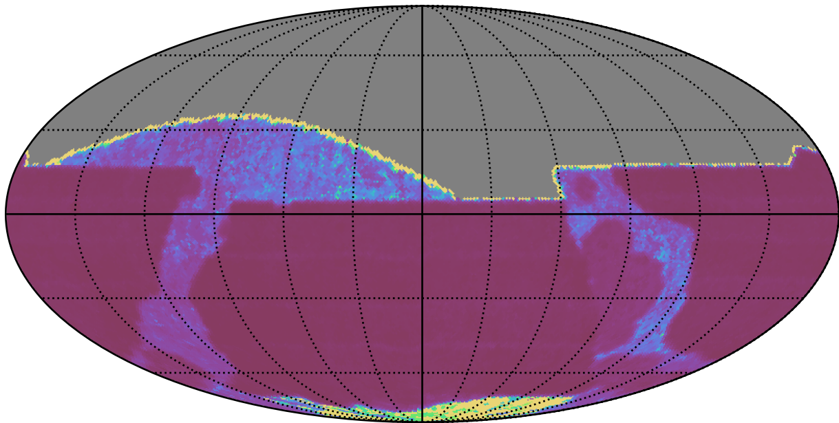
too_5_1v3.4_10yrs All sky z band: Median Inter-Night Gap
