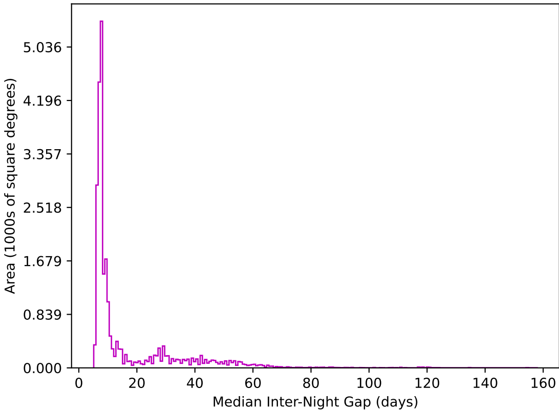
too_5_1v3.4_10yrs All sky z band: Median Inter-Night Gap
