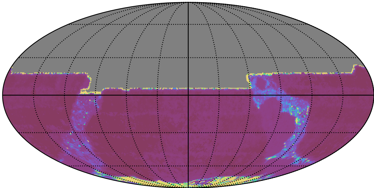
too_5_1v3.4_10yrs All sky y band: Median Inter-Night Gap
