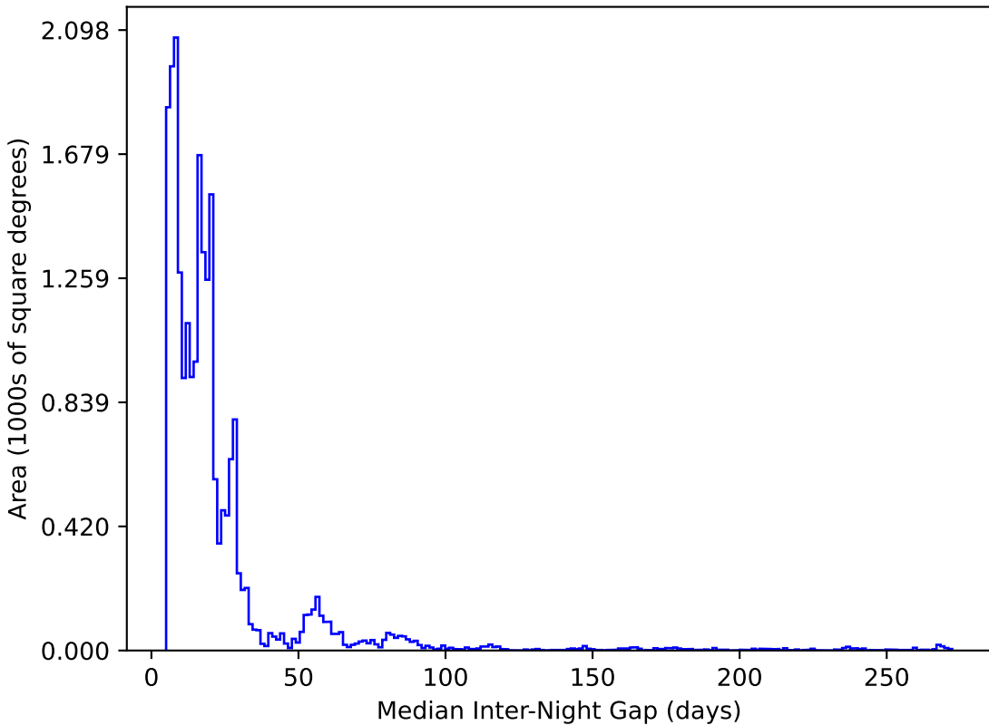
too_5_1v3.4_10yrs All sky y band: Median Inter-Night Gap
