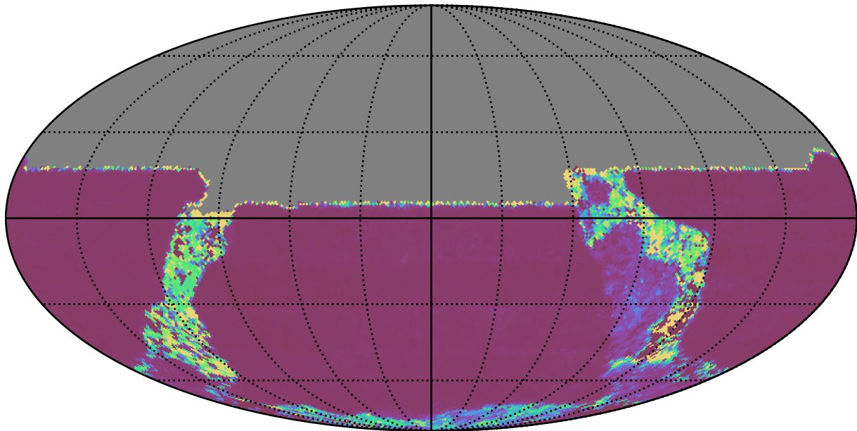
too_5_1v3.4_10yrs All sky u band: Median Inter-Night Gap
