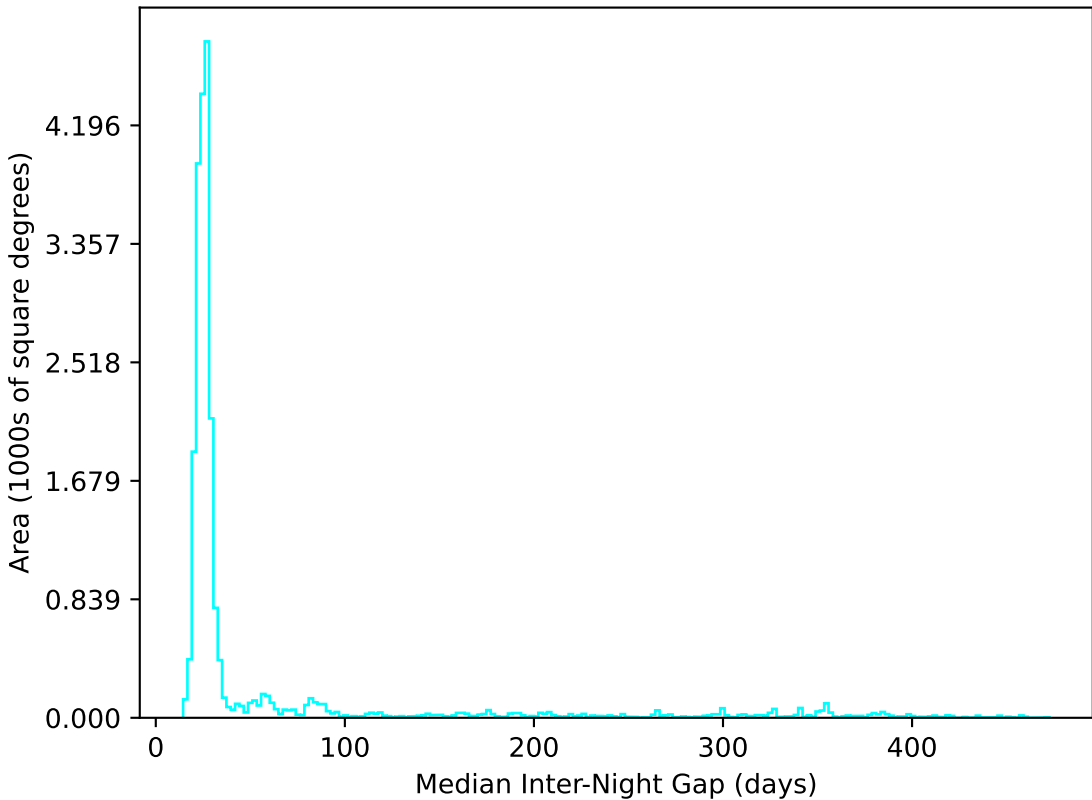
too_5_1v3.4_10yrs All sky u band: Median Inter-Night Gap
