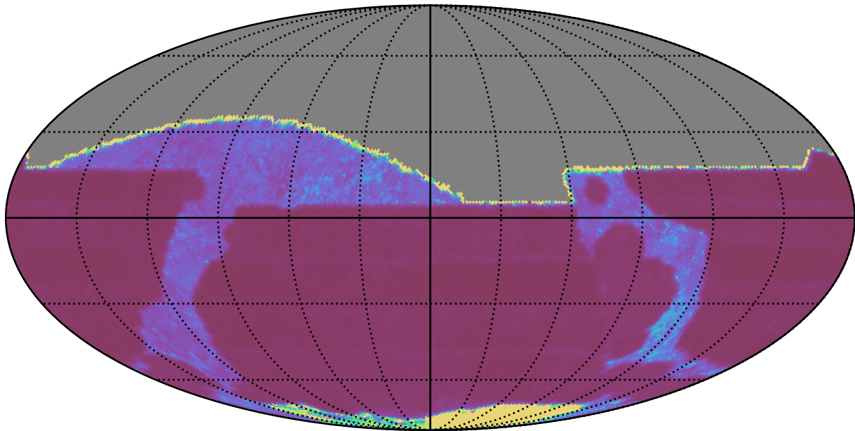
too_5_1v3.4_10yrs All sky r band: Median Inter-Night Gap
