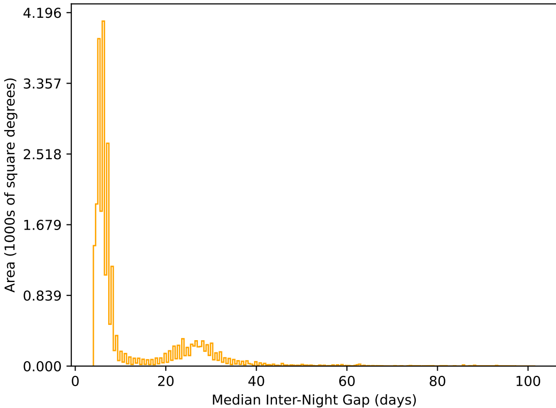
too_5_1v3.4_10yrs All sky r band: Median Inter-Night Gap
