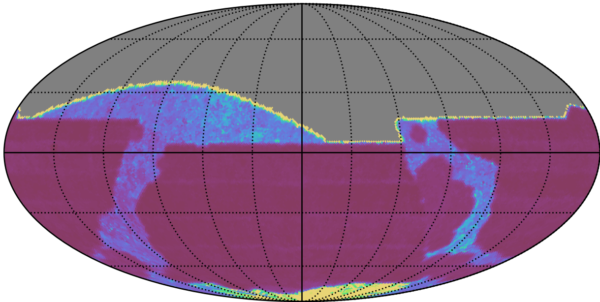
too_5_1v3.4_10yrs All sky i band: Median Inter-Night Gap
