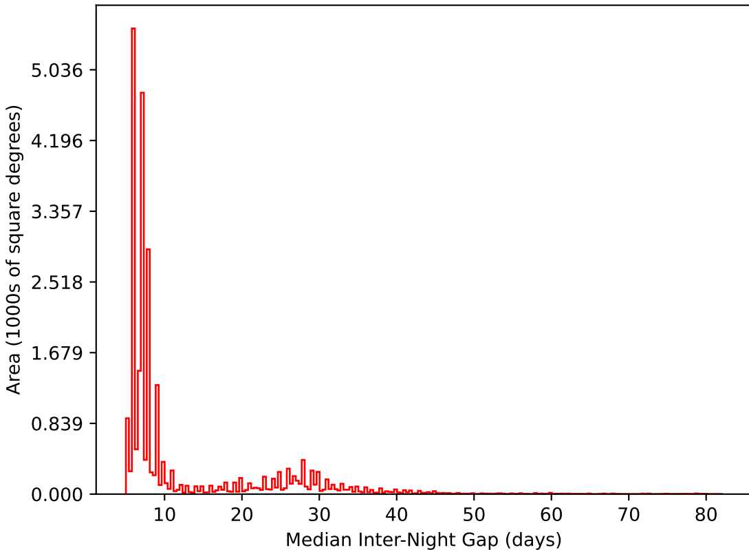
too_5_1v3.4_10yrs All sky i band: Median Inter-Night Gap
