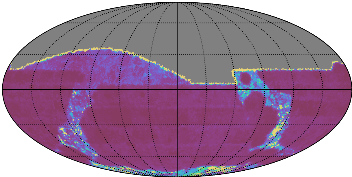
too_5_1v3.4_10yrs All sky g band: Median Inter-Night Gap
