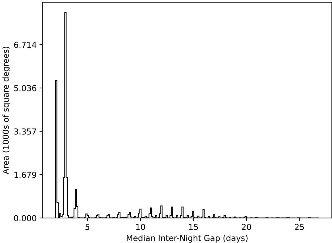
too_5_1v3.4_10yrs All sky all bands: Median Inter-Night Gap
