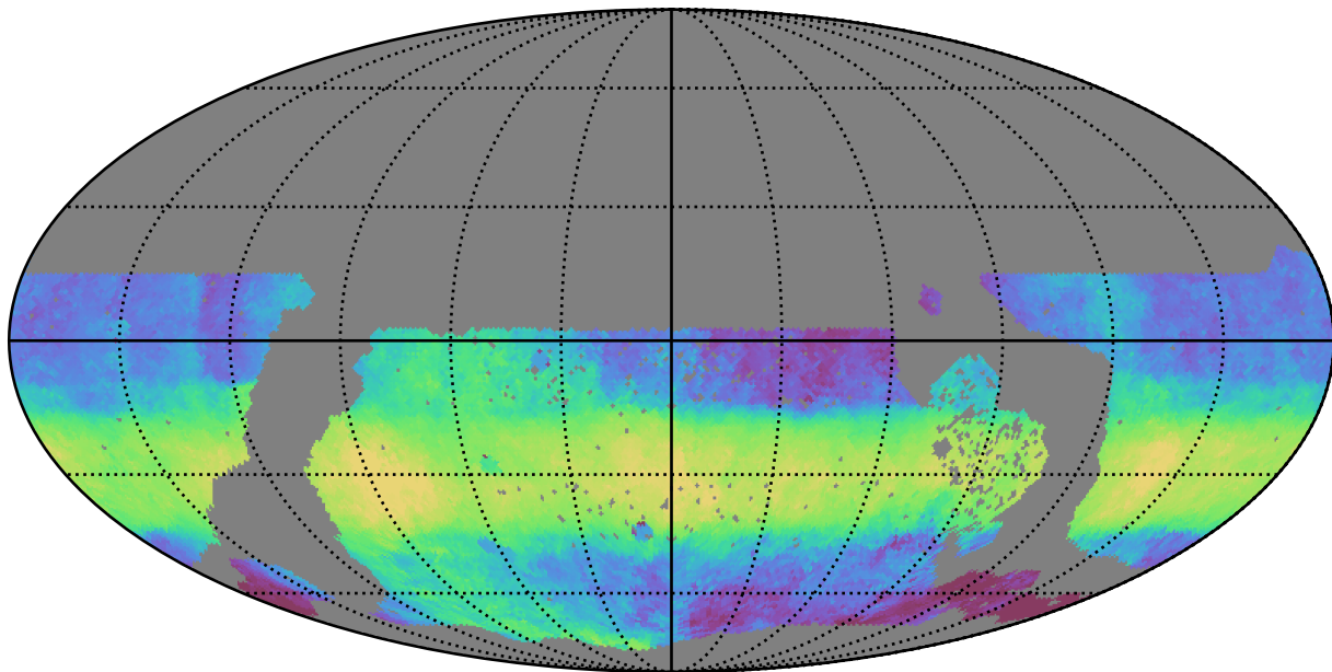
too_5_1v3.4_10yrs WFD z band: Median HA
