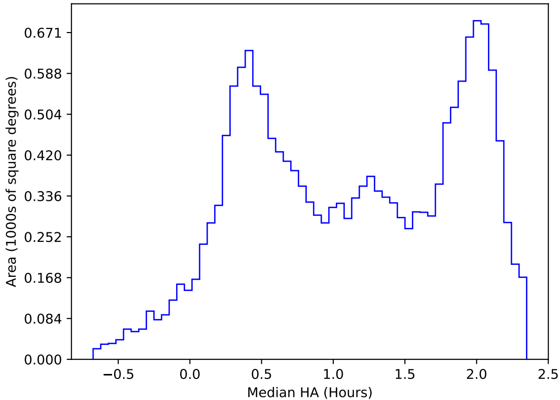
too_5_1v3.4_10yrs WFD z band: Median HA
