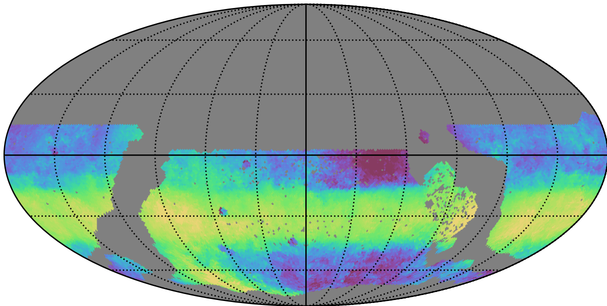
too_5_1v3.4_10yrs WFD y band: Median HA
