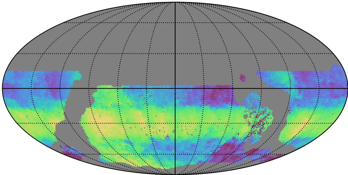
too_5_1v3.4_10yrs WFD u band: Median HA
