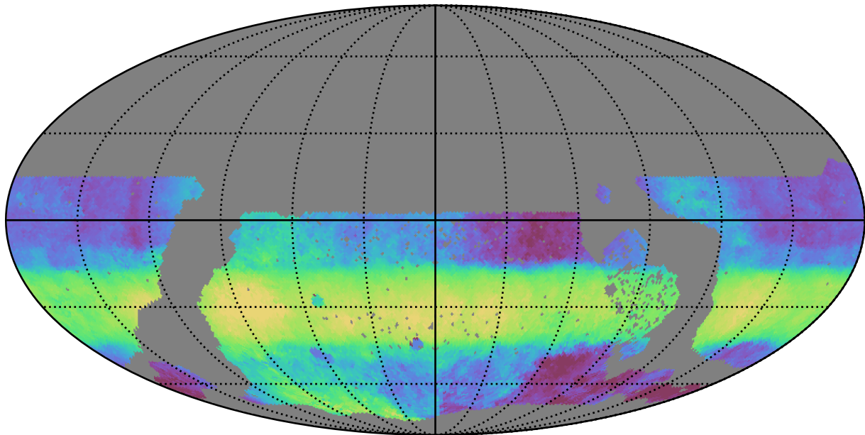
too_5_1v3.4_10yrs WFD r band: Median HA
